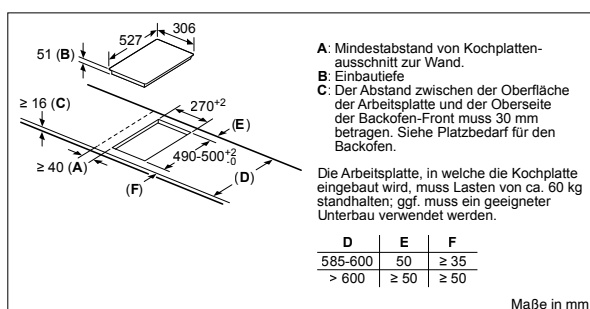
PIB375FB1E – Comfort Profil
