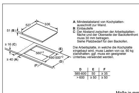
PXY675DC1E – Comfort Profil
