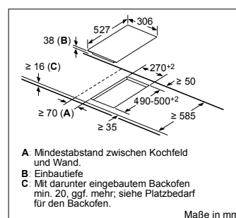
PKF375FP2E – Comfort Profil
