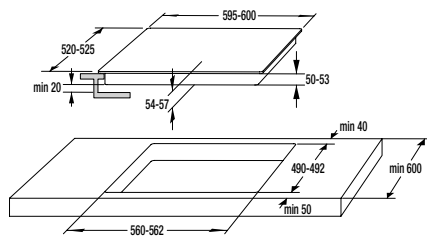
ECS 646 BCSC / ECT 643 BSC / ECT 643 BX / ECT 43 X / ECT 43 X
