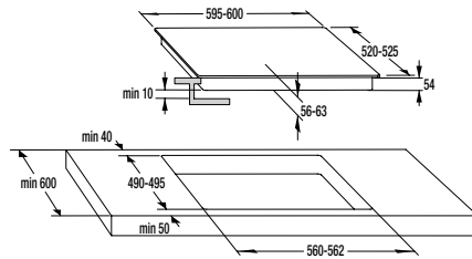
IT 640 BX / IT 640 BSC / IT 640 WSC / ID 640 X / IT 40 SC / ID 64 BX
