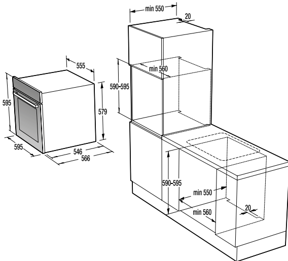
BCS 798 S24BG / BCS 798 S24X / BCS 747 S34X
