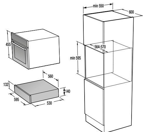
WD 1410 X / WD 1410 B
