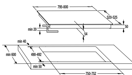
IS 846 BG / IT 843 BX
