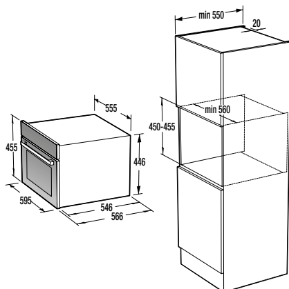
BCMS 598 S19X / BCS 598 S24BG / BCM 598 S18X BCM 4547 A10X / BCM 4547 A10BG
